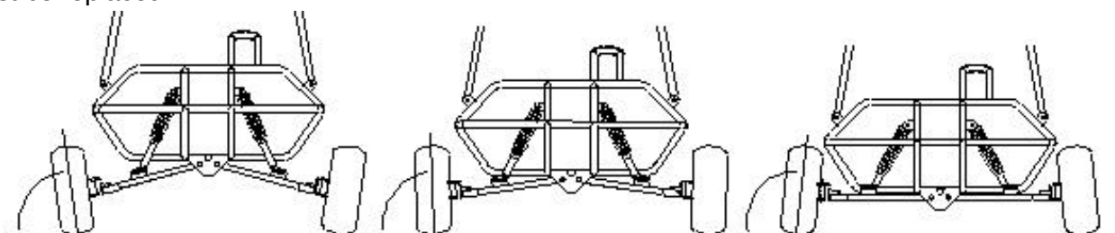
A. EXTREME OUTWARD CAMBER (NEW SHOCKS, NOT BROKEN IN) B. SLIGHT OUTWARD CAMBER (SHOCKS BROKEN IN) C. INWARD CAMBER (SHOCKS NEED TO BE ADJUSTED OR REPLACED)
