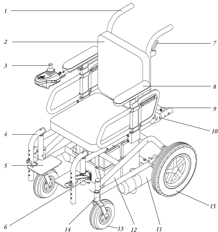
Quickie Z-500
