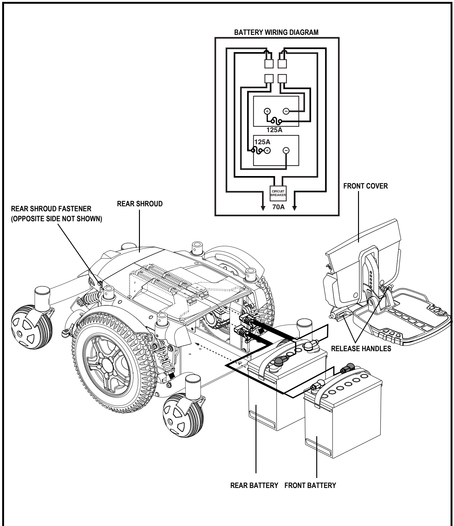
Figure 27. Battery Installation
