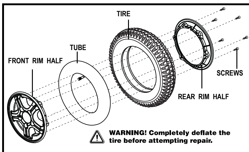
Figure 26. Quantum 6000Z Series Drive Wheel Disassembled
