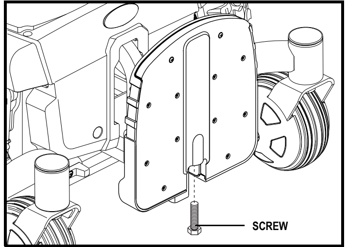
Figure 23. Underside of Foot Platform
