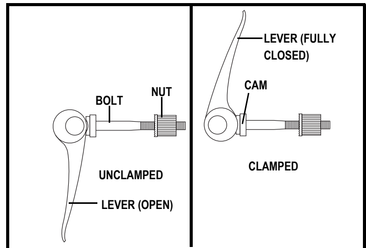
Figure 22. Quick Release Fastener Operation
